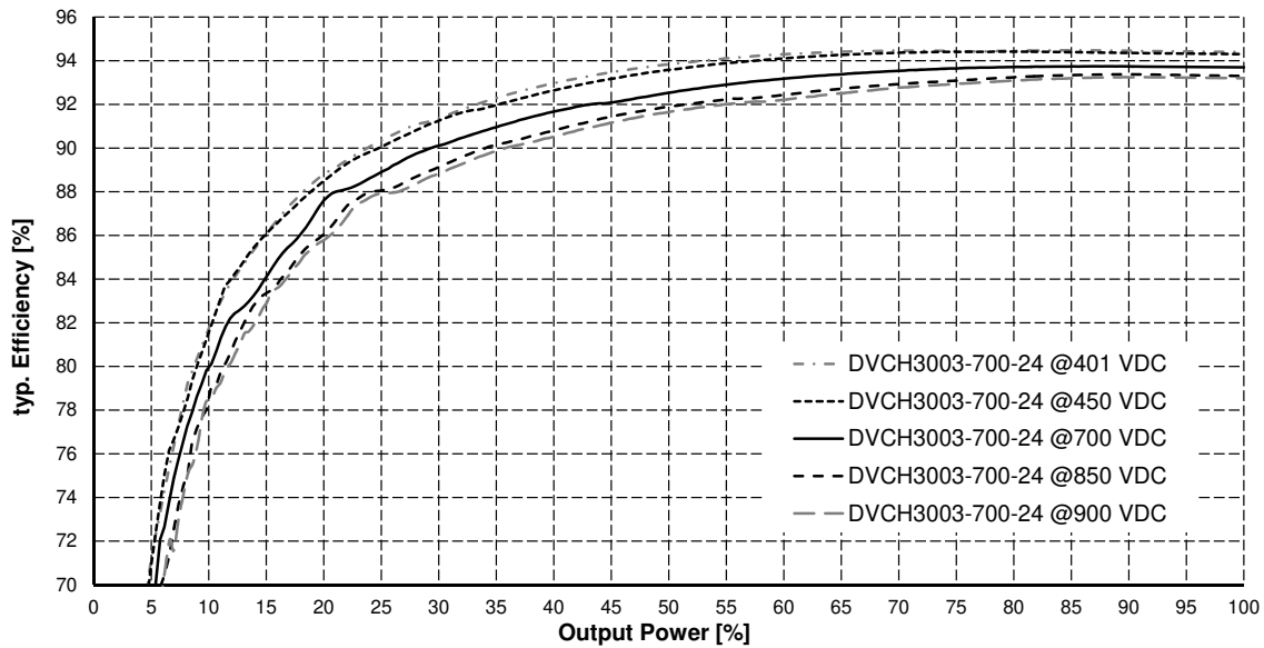
Figure 9.3: Efficiency as a function of output power
