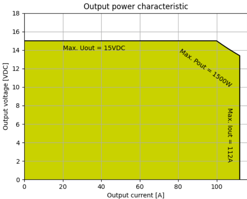
Figure 9.4: Output power DVCH1503-400-12
